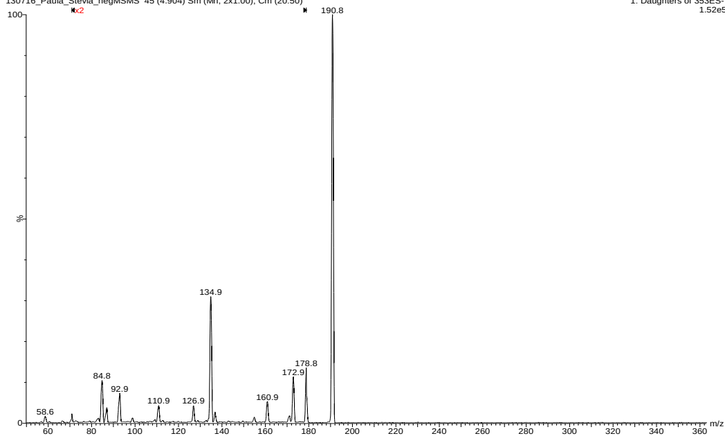
Fig. 12: Chlologenic acid.
