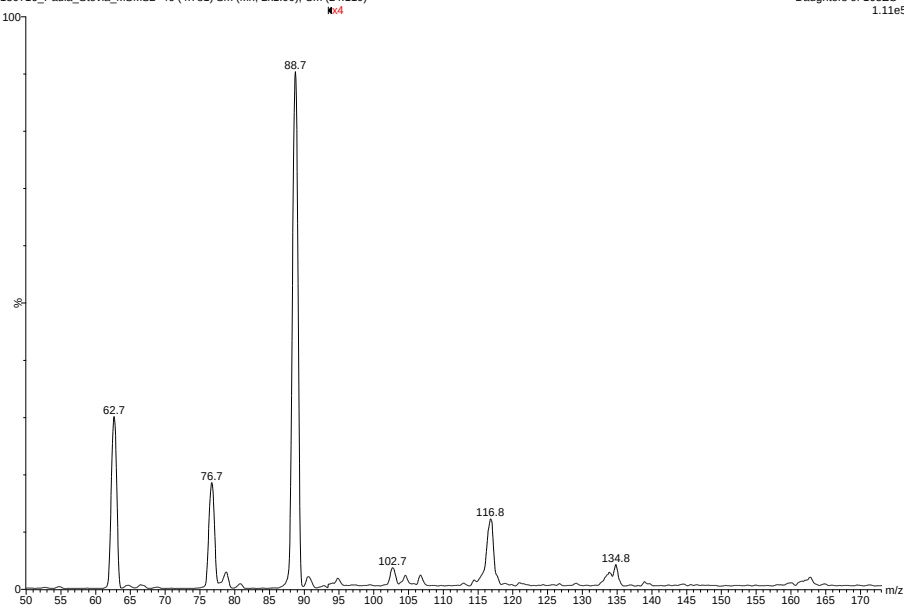
Fig. 4: Caffeic acid
