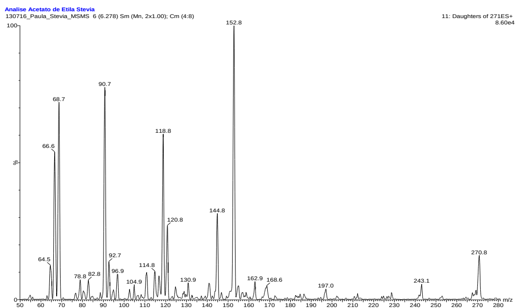
Fig. 9: Apigenin
