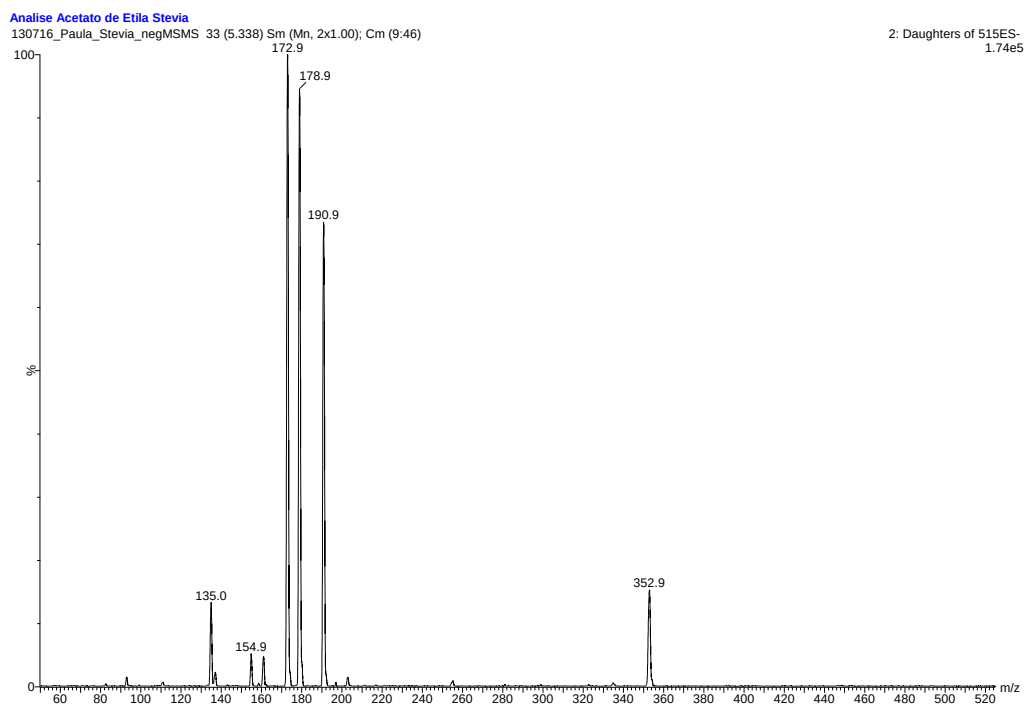
Fig. 13: Dicafeoylquinic acid.
